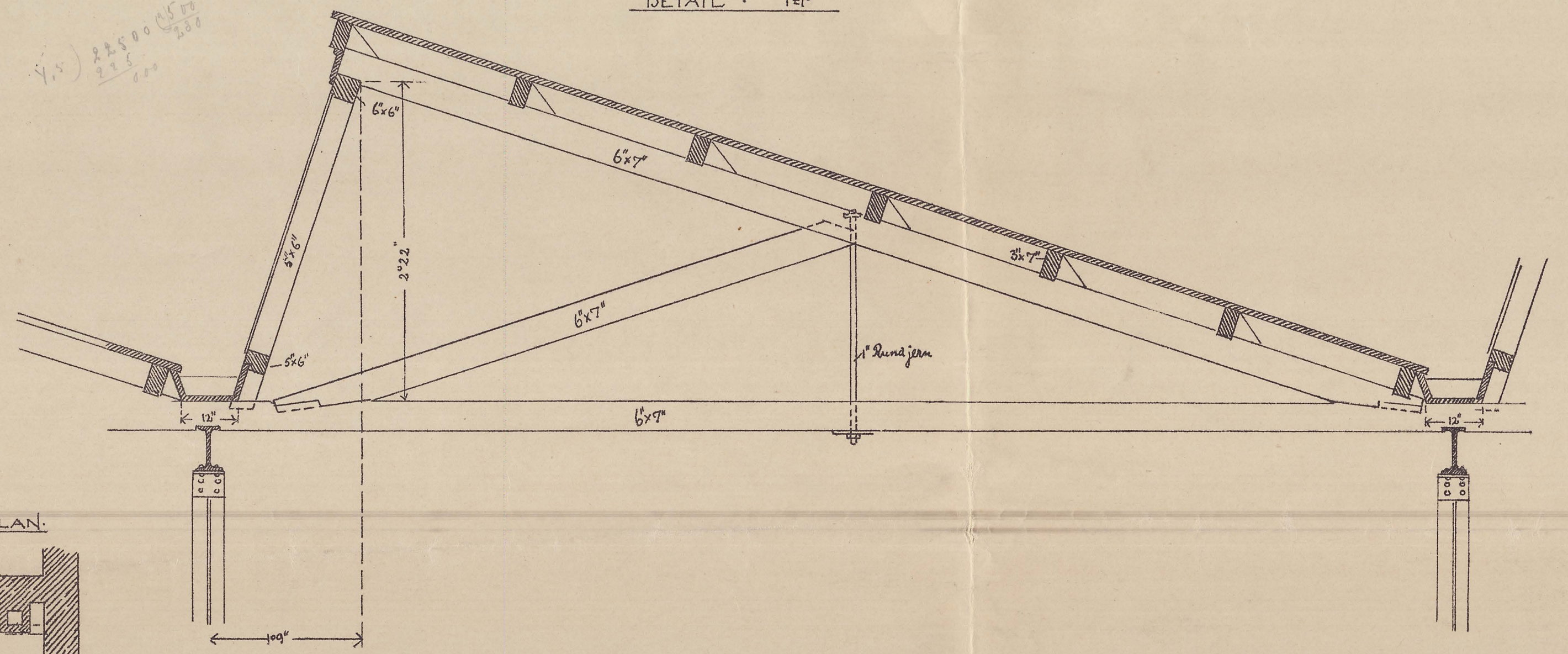
DETAIL 1:6
