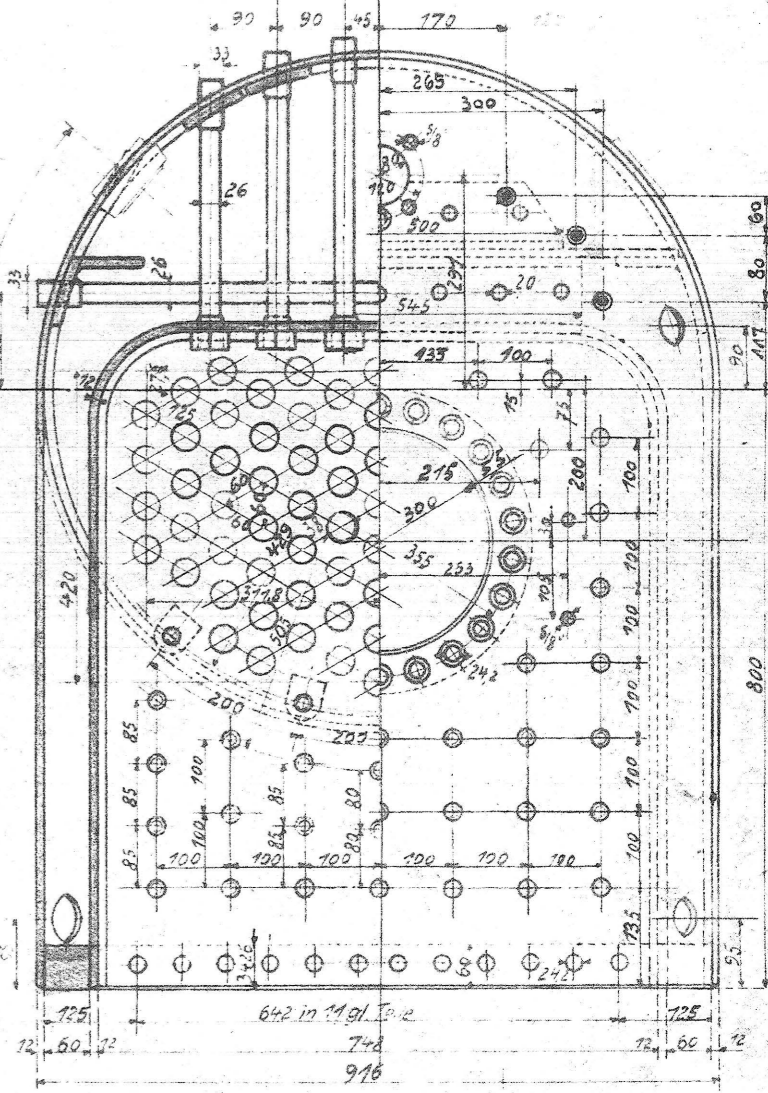
82 Heizrohre
