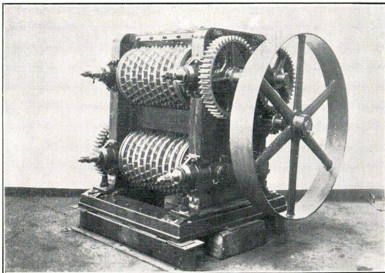
KULKNUSER - KAPACITET: 50 TONS PR. TIME COAL BREAKER - CAPACITY: 50 TONS PER HOUR
