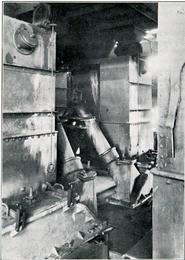
W-D KONTINUERLIG VERTIKALOVN - GASAFGANG W-D CONTINUOUS VERTICAL RETORT OVEN - GAS OFFTAKE
