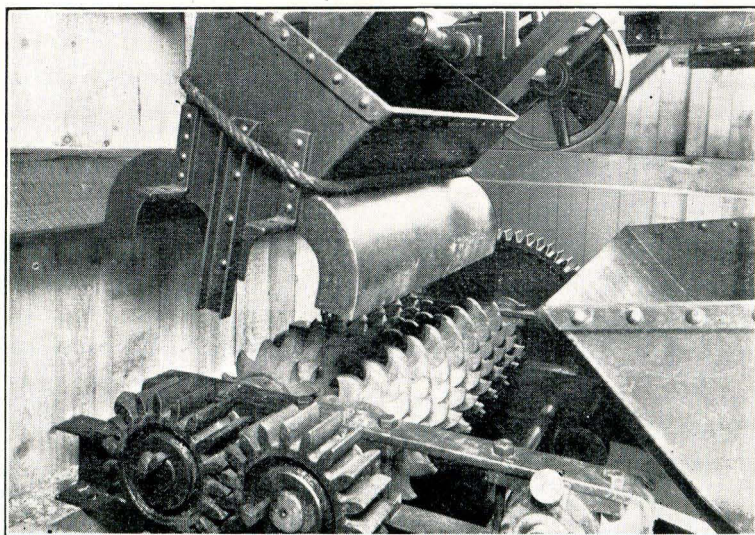
KOKSKNUSER - KAPACITET: 15 TONS PR. TIME COKE BREAKER - CAPACITY: 15 TONS PER HOUR
