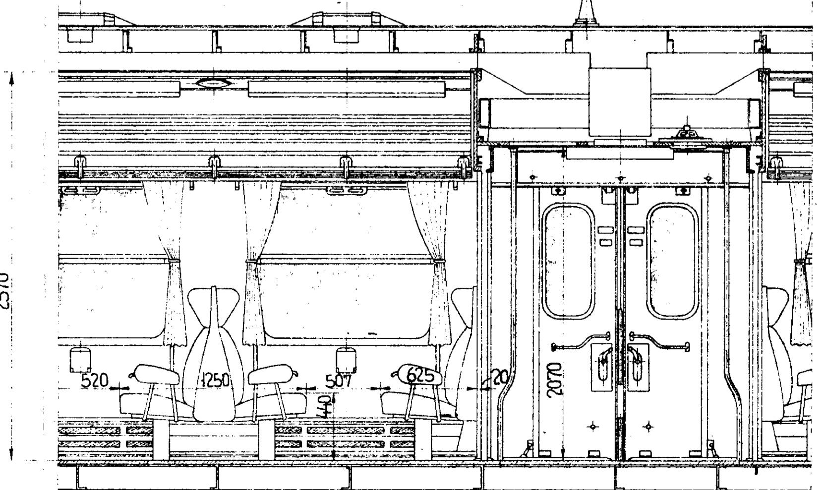
Snit C-C.
