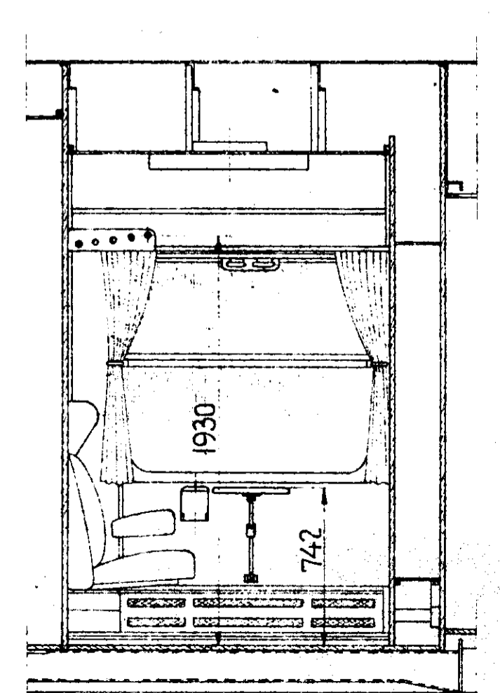
Snit D-D.
