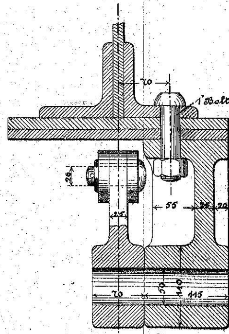
Laaseaxel.
